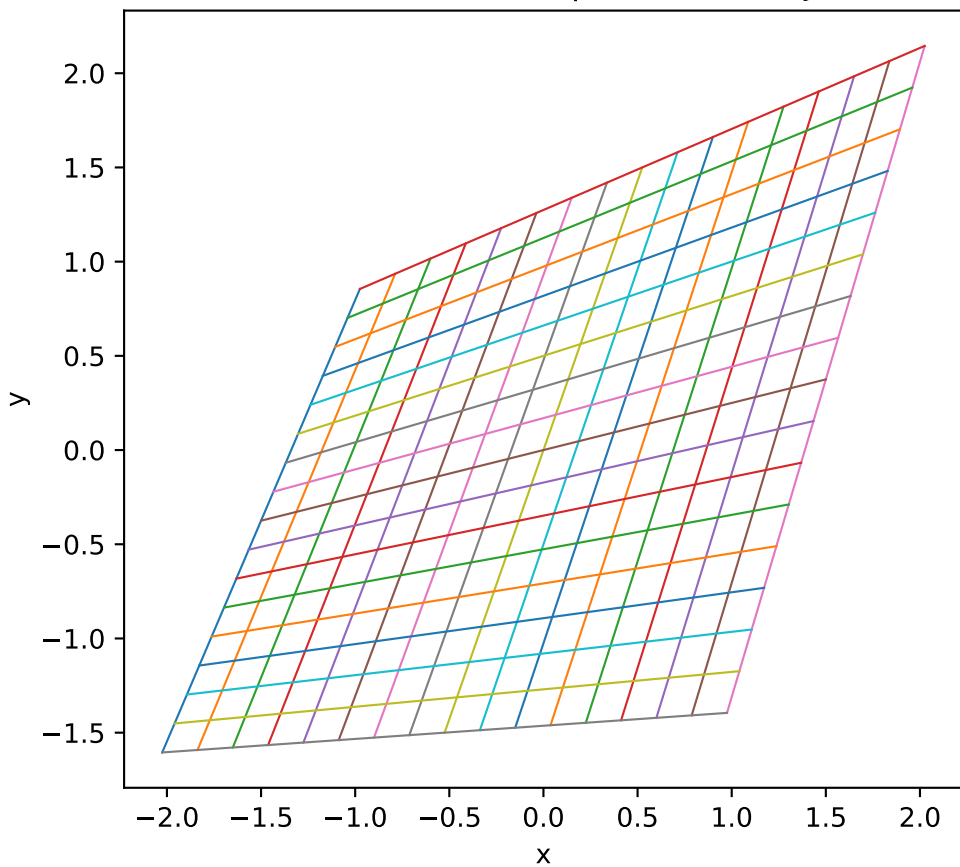
A nonlinear coordinate map and its local Jacobian
