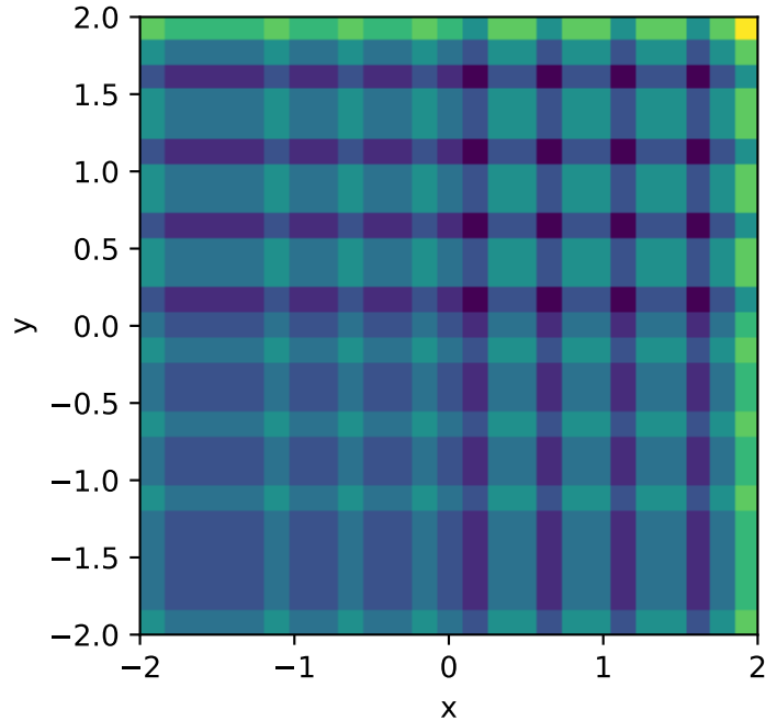
Numerical curl
