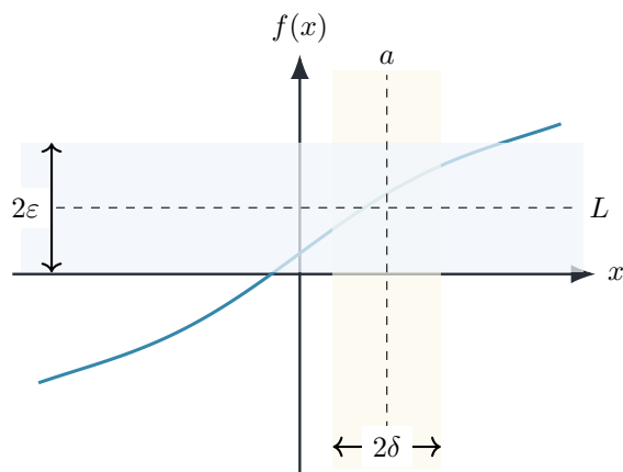
Figure 2.10: The \epsilon - \delta definition controls output error by restricting the input to a sufficiently small neighborhood.
