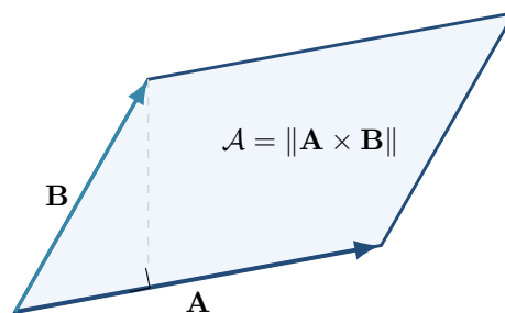
Figure 1.14: The cross-product magnitude equals the area of the parallelogram spanned by the two vectors.
