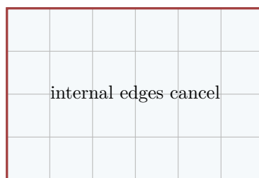
Figure 3.12: Green's theorem: internal edge contributions cancel when small cells are assembled, leaving only the outer boundary.
