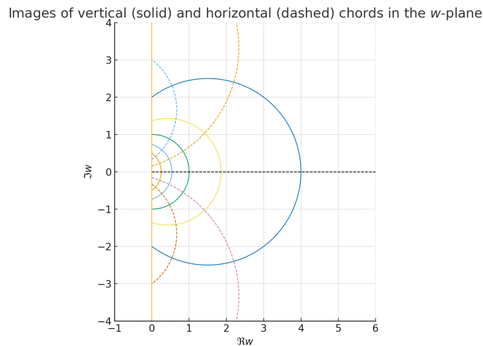
Figure 7: Images of the chords from Figure ?? under the Cayley transform. Each chord becomes a generalized circle lying in the right half-plane; the real axis segment maps to the positive real axis.
