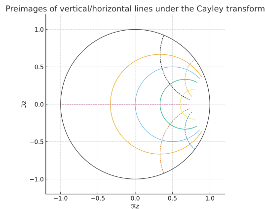
Figure 5: Preimages in the z -plane of the vertical and horizontal lines from Figure ?? . Vertical lines become circles orthogonal to the unit circle, while horizontal lines become circles tangent to \partial\mathbb{D} at z = 1 .
