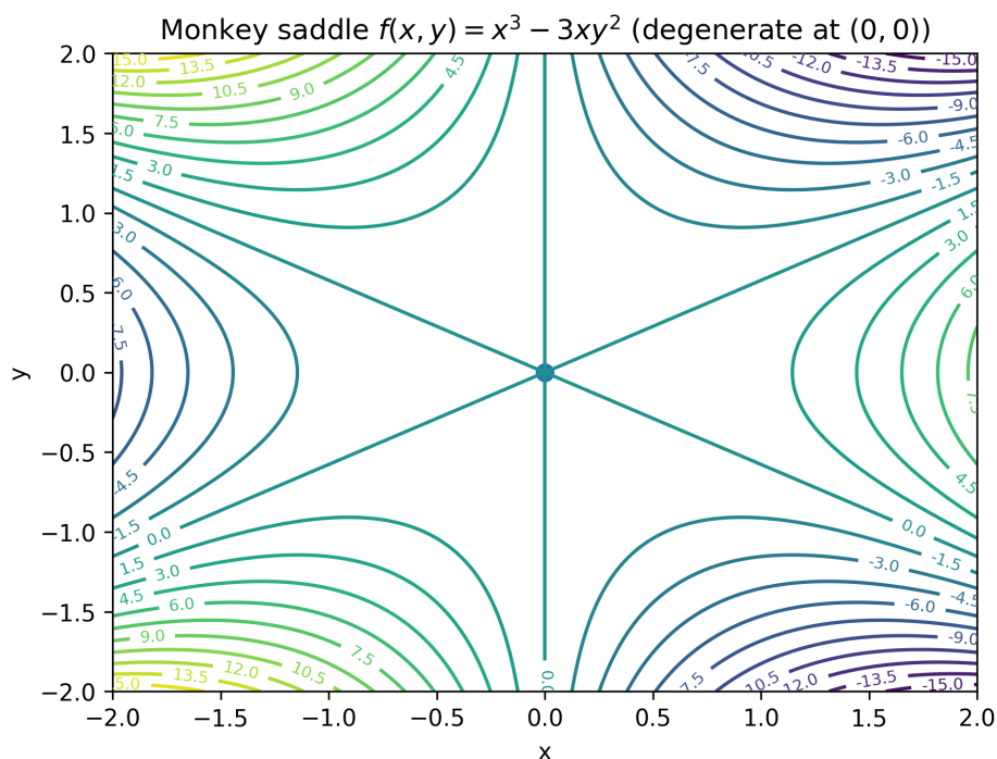
Figure 29: Example of a degenerate critical point: the monkey saddle f(x, y) = x^3 - 3xy^2 has a critical point at (0, 0) with degenerate Hessian.
