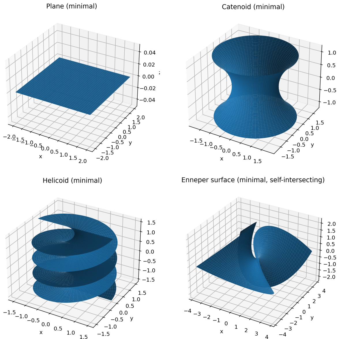
Figure 7: Classic minimal surfaces: plane, catenoid, helicoid, Enneper.
