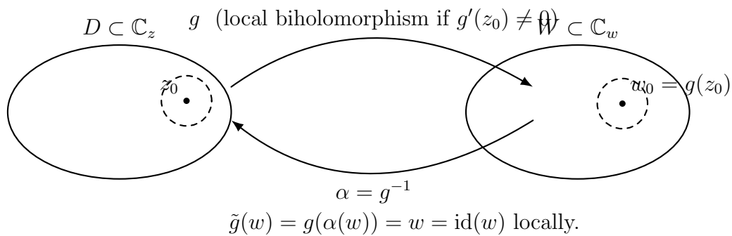
Figure 10: Local normalization near a regular point: if g'(z_0) \neq 0 , choose \alpha = g^{-1} so that \tilde{g} = \text{id} .
