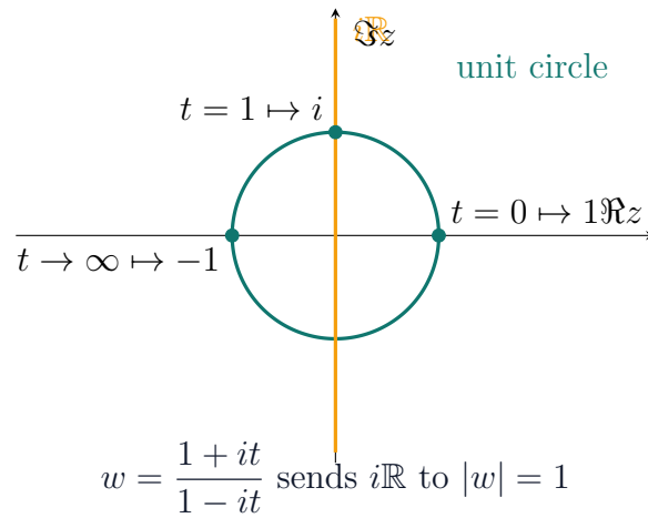
Figure 4: Cayley transform: eigenvalues of skew-Hermitian matrices (imaginary axis) map to unit-modulus eigenvalues (unit circle).
