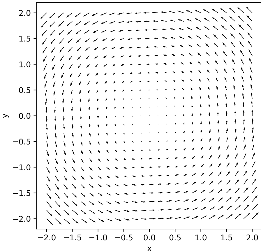
Rotational field F=(-y,x)
