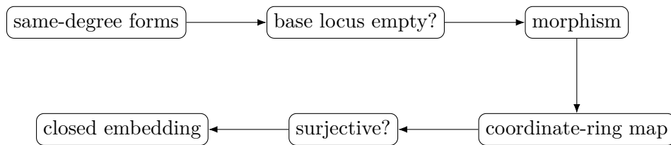
Figure 38.8: A practical workflow for turning homogeneous coordinate formulas into scheme-theoretic projective morphisms and embeddings.
