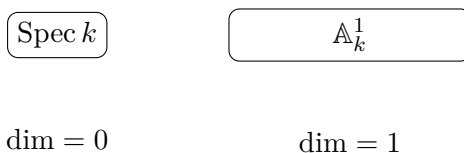
Figure 30.3: AG8 Problem 3(d): a nonempty open component can have smaller dimension than the whole scheme.
