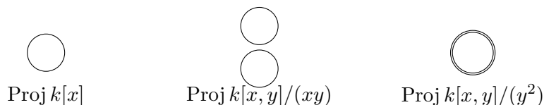
Figure 35.8: \operatorname{Proj} can be one reduced point, two reduced points, or a one-point nonreduced scheme.
