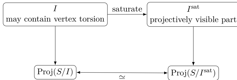
Figure 37.5: Saturation removes homogeneous algebra supported only at the irrelevant cone vertex and leaves the projective scheme unchanged.
