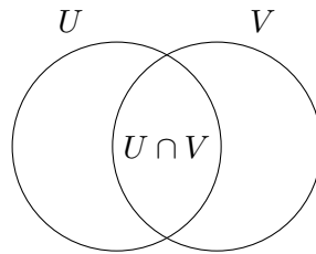
Figure 46.5: For a two-open cover, the first Čech obstruction lives on the overlap.
