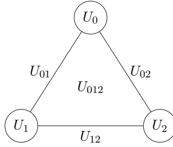
Figure 47.4: The nerve of a three-open cover: vertices, edges, and a 2-simplex encode the first three Čech degrees.
