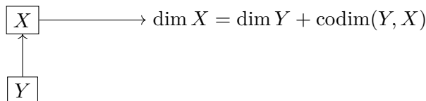
Figure 31.5: For varieties, ambient dimension splits into subvariety dimension plus codimension.
