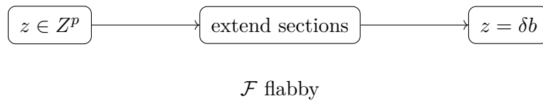
Figure 47.6: Flabbiness kills positive-degree Čech cocycles by successive extension.
