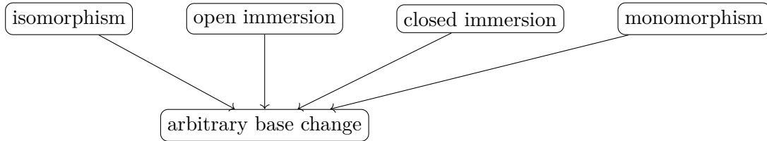
Figure 24.6: Elementary morphism classes proved stable under base change in VI/24.
