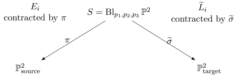
Figure 45.6: The common resolution of the standard quadratic Cremona transformation.
