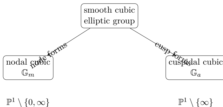
Figure 43.7: The two basic singular degenerations of an elliptic group law.
