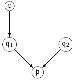
Figure 11.3: The local spectrum retains the generalizations of the chosen point.
