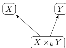
Figure 30.8: Under suitable geometric-integrality hypotheses, dimensions add in products of varieties.
