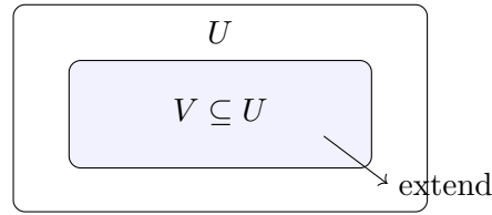
Figure 46.1: Flabbiness says every section on the smaller open extends to the larger open.
