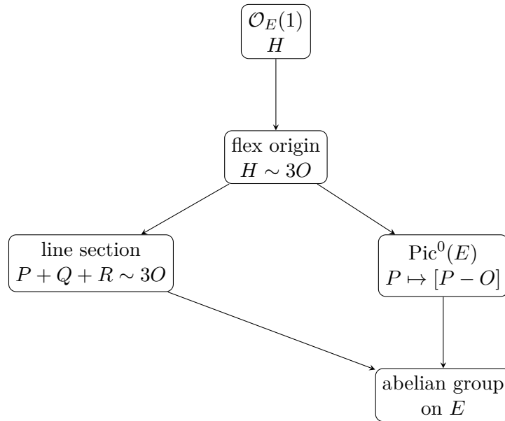
Figure 43.8: The flex-origin dictionary that turns degree-three plane geometry into degree-zero Picard addition.
