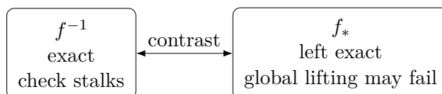
Figure 16.10: Inverse and direct image have different exactness behavior.
