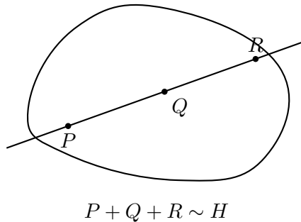
Figure 43.3: A line cuts a cubic in a divisor of degree three. Multiplicities replace distinct points in tangent cases.
