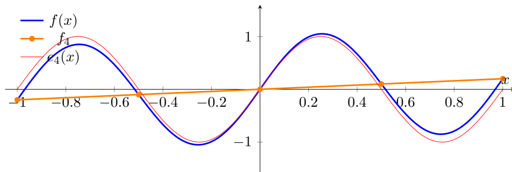
Figure 1: Interpolation and error for n = 4 .
