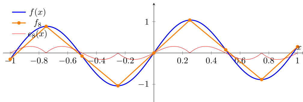
Figure 1: Interpolation and error for n = 8 .
