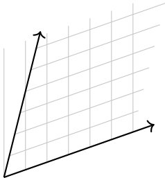
transformed basis
