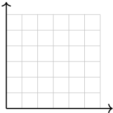
original basis
