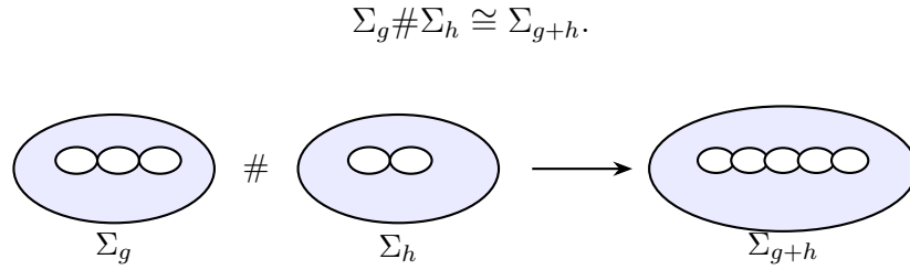
Figure 6: For orientable surfaces, connected sum adds handles: \Sigma_g \# \Sigma_h \cong \Sigma_{g+h} .
