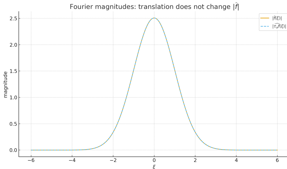
Figure 19: Magnitudes of the Fourier transforms |\widehat{f}(\xi)| and |\widehat{\tau_a f}(\xi)| . They coincide, which reflects the identity \widehat{\tau_a f}(\xi) = e^{-ia\xi} \widehat{f}(\xi) : translation in x only affects the phase, not the magnitude, of the Fourier transform.
