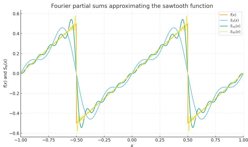
Figure 31: Global comparison of the sawtooth function f and partial sums S_N of its sine series for N = 3, 10, 50 .
