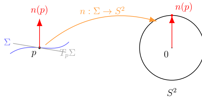
Figure 6: The Gauss map assigns to each point p \in \Sigma its unit normal vector n(p) , viewed as a point on the unit sphere S^2 .
