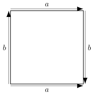
Figure 24: Fundamental polygon for the Klein bottle. Traversal yields a b a b^{-1} .
