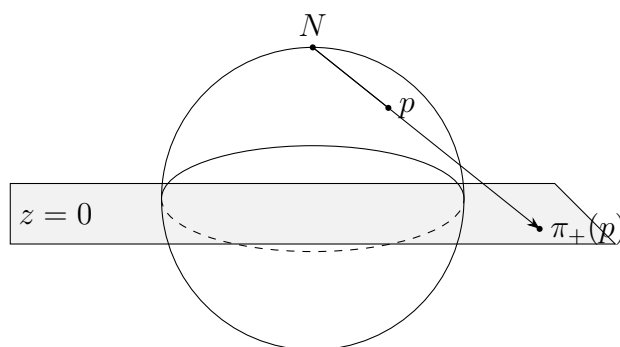
Figure 15: Stereographic projection \pi_+ from the north pole N onto the plane z = 0 .
