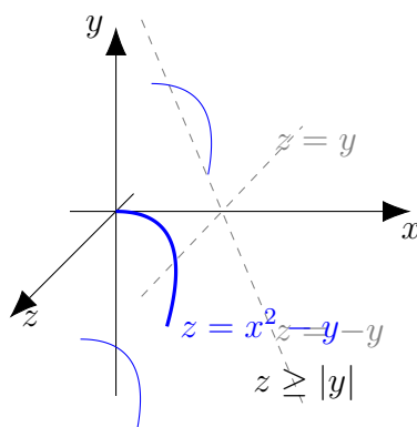
Figure 40: Schematic sketch of the image of \sigma(u, v) = (u + v, 2uv, u^2 + v^2) : a parabolic sheet z = x^2 - y cut by z \geq |y| .
