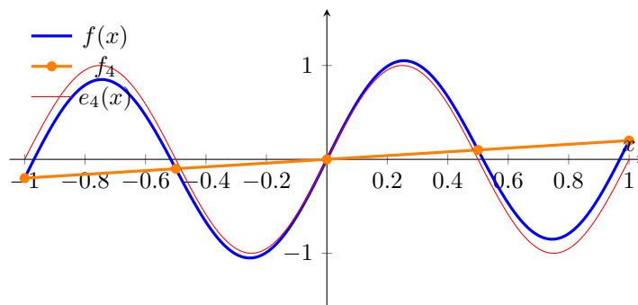
Figure 1: Interpolation and error for n = 4 .
