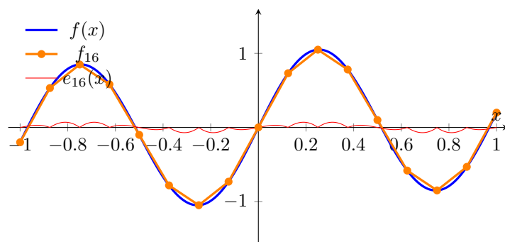
Figure 3: Interpolation and error for n = 16 .
