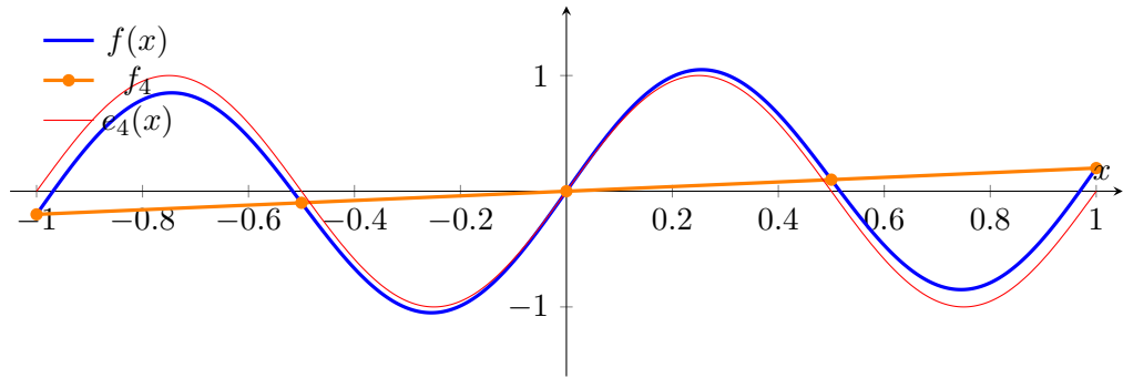
Figure 1: Interpolation and error for n = 4 .
