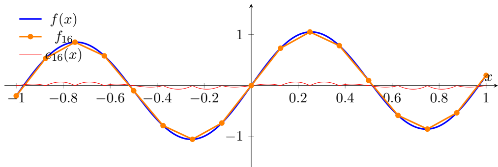
Figure 3: Interpolation and error for n = 16 .
