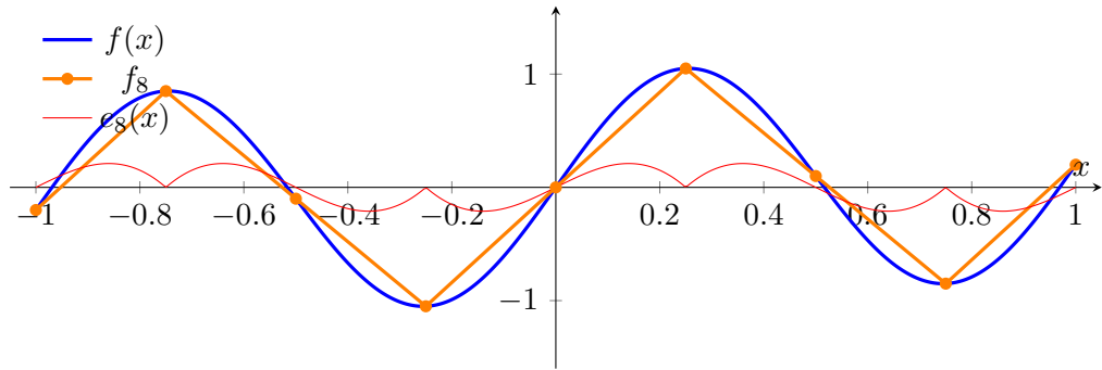
Figure 2: Interpolation and error for n = 8 .
