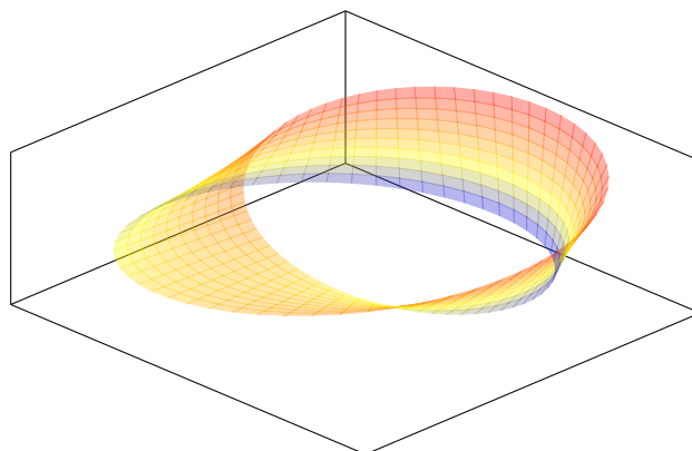
Figure 7: The Möbius strip: total space of the Möbius line bundle over S^1 .
