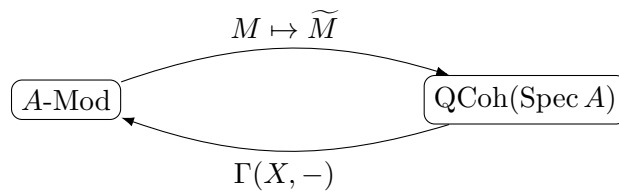
Figure 33.5: On an affine scheme, modules and quasi-coherent sheaves contain the same information.
