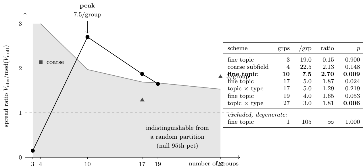
Figure 2: Spread ratio against grouping granularity, 105 probe problems, 2000 permutation draws per arm, seed 20260905. The shaded region is each granularity’s own null 95th percentile expressed as a ratio, so a point inside it is indistinguishable from a size-matched random partition; at three groups that band runs off the top of the axis at 4.25. The band narrows as groups get finer — 3.00 at four groups, 1.97 at ten, 1.53 at twenty-seven — which is the whole of the effect described below. Circles are the fine-topic arm at five pooling thresholds, the square is the four coarse subfields, triangles cross the topic label with the answer type. The dashed line at 1 is “no structure”.
