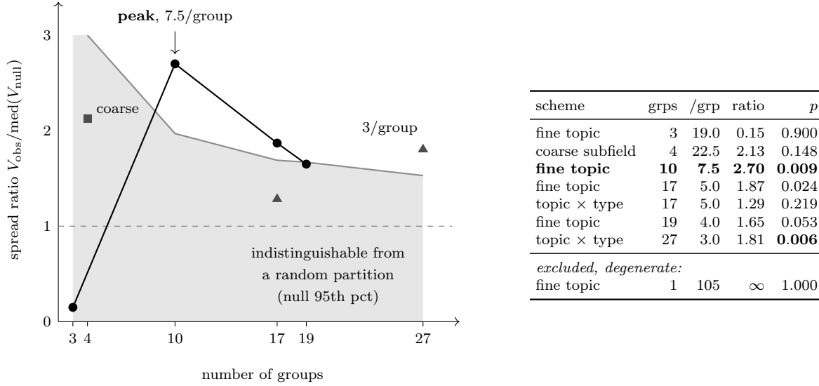
Figure 2: Spread ratio against grouping granularity, 105 probe problems, 2000 permutation draws per arm, seed 20260905. The shaded region is each granularity’s own null 95th percentile expressed as a ratio, so a point inside it is indistinguishable from a size-matched random partition; at three groups that band runs off the top of the axis at 4.25. The band narrows as groups get finer — 3.00 at four groups, 1.97 at ten, 1.53 at twenty-seven — which is the whole of the effect described below. Circles are the fine-topic arm at five pooling thresholds, the square is the four coarse subfields, triangles cross the topic label with the answer type. The dashed line at 1 is “no structure”.
