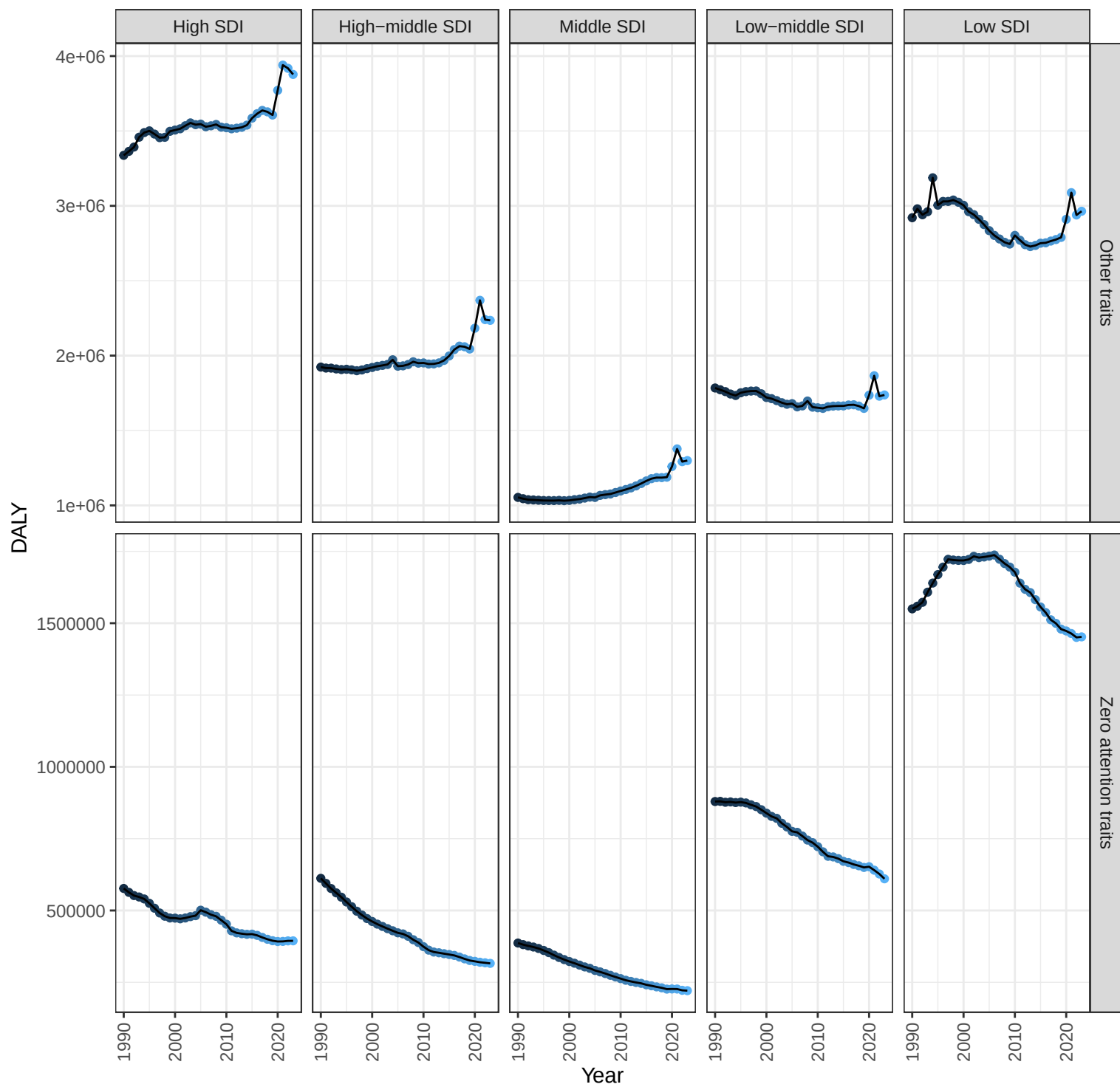
DALY trends of zero and non-zero attention traits
