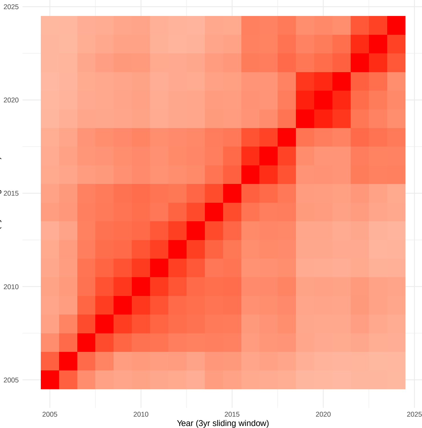
Correlation of Total Attention Scores between Time Strata
