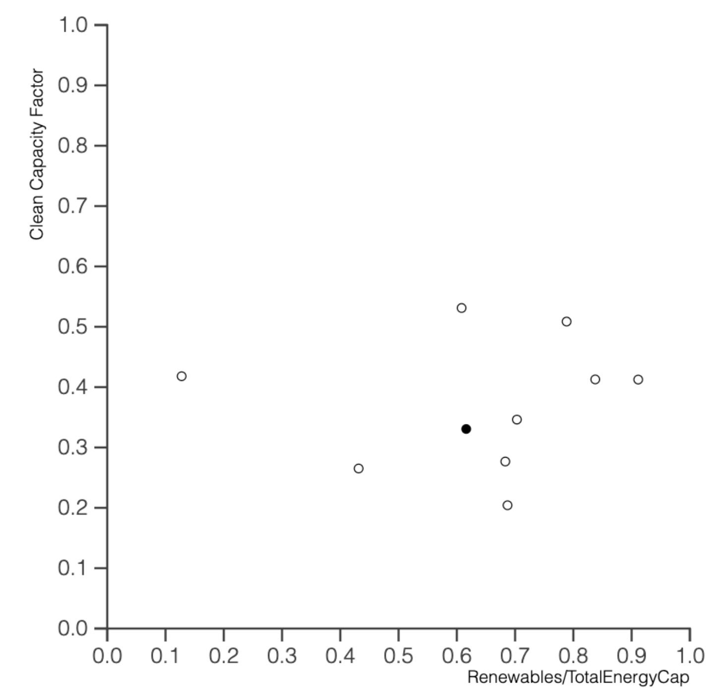
Clean energy efficiency against proportion of renewable energy cap
