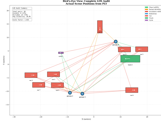
Figure 8. Bird’s-eye view visualization of line-of-sight analysis showing visibility rays from pedestrians to vehicles. Green rays indicate clear LOS ( \geq 60\% visibility), orange indicates partial visibility (40-60%), and red indicates occluded paths ( < 40\% ).
