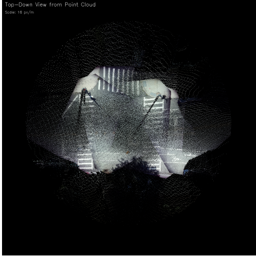
Figure 3. Pi3 dense 3D point cloud reconstruction with camera poses
