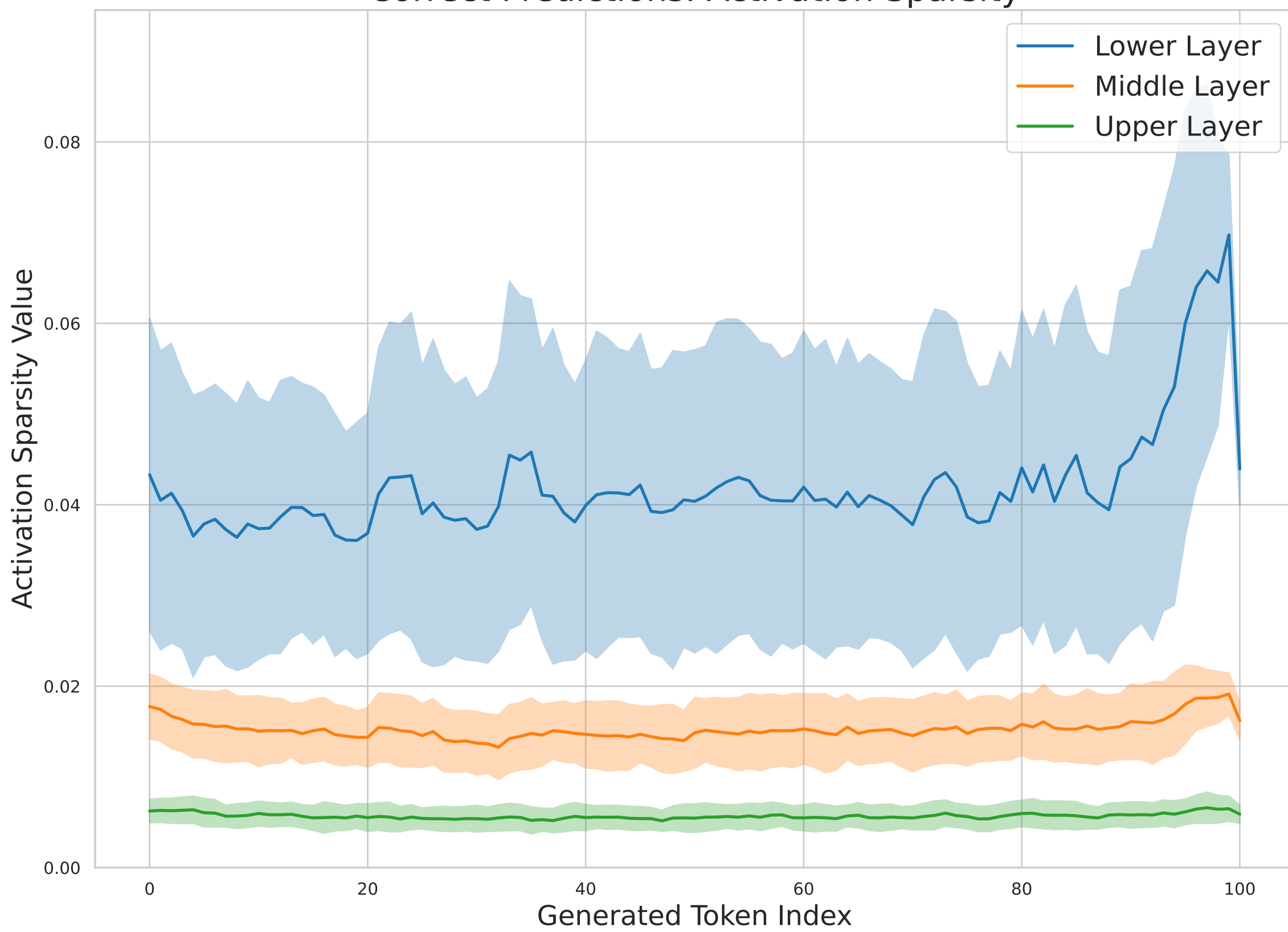
Correct Predictions: Activation Sparsity
