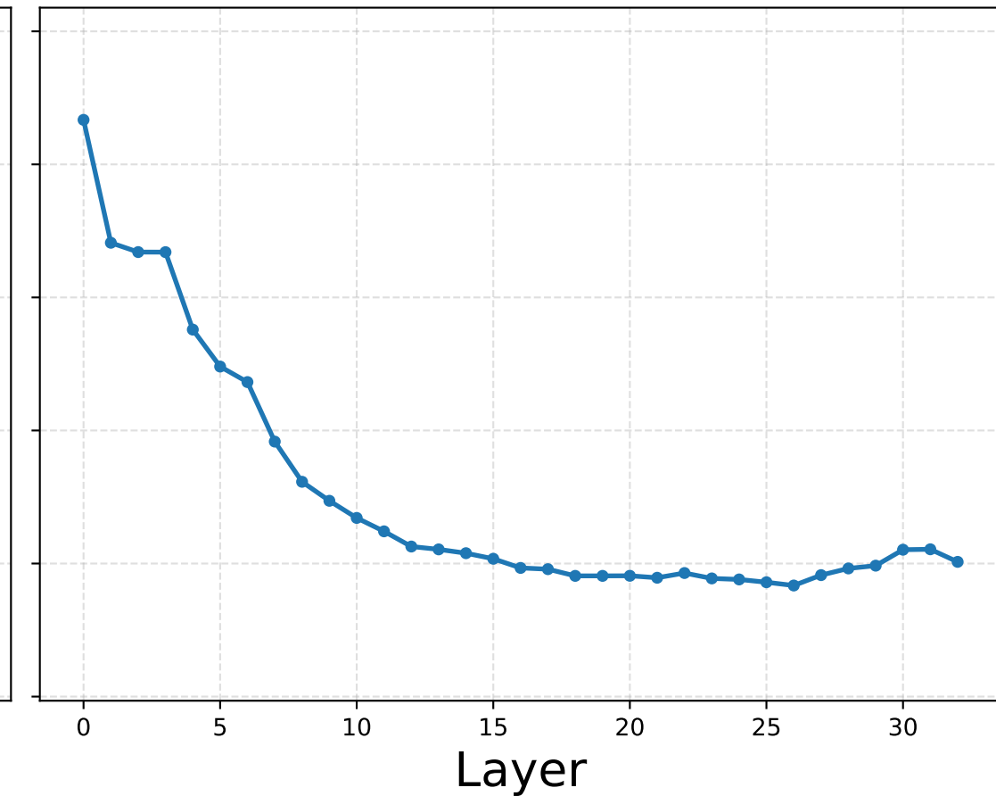
Olmo-3-7B-Instruct
