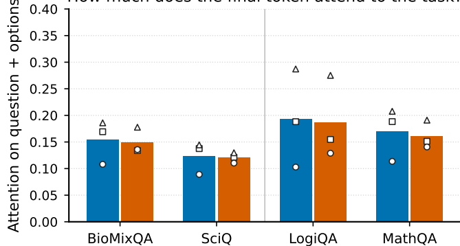
How much does the final token attend to the task?
