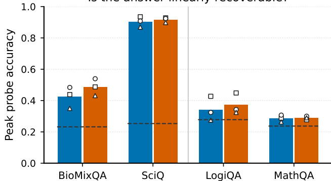
Is the answer linearly recoverable?
