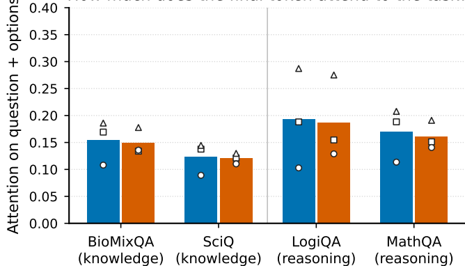
How much does the final token attend to the task?
