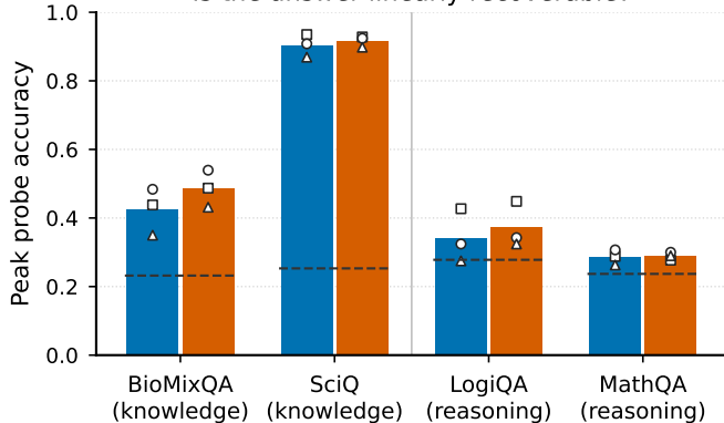
Is the answer linearly recoverable?
