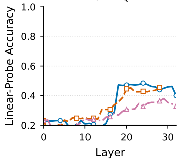
BioMixQA
