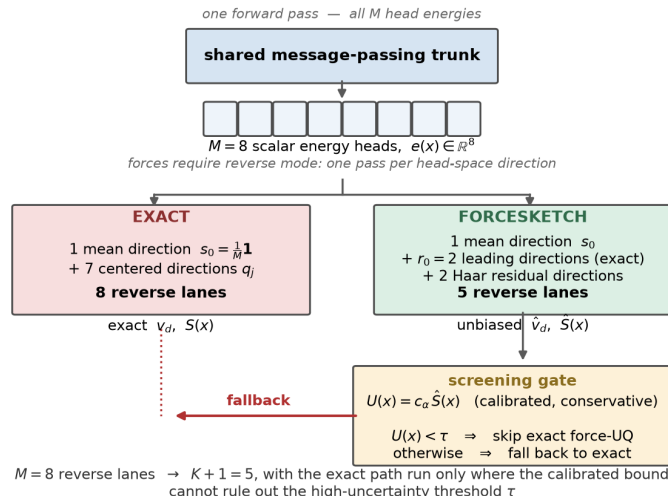
Figure 3: What ForceSketch replaces. All M head energies come from one forward pass, but forces do not: exact disagreement needs the full centered head subspace, M lanes. ForceSketch spends K+1 , and — since that is not accurate enough to replace exact uncertainty at K \leq 4 under either acquisition rule (Section 5.1) — its score feeds a calibrated gate that runs the exact path only where the bound cannot rule out the threshold. Whether fewer lanes also cost less time depends on the autodiff regime (Section K.1).
