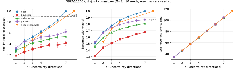
Figure 4: Accuracy and cost against K , ranked by the global statistic S . Latency curves coincide for every method at equal lane count under the serial implementation; batched reverse mode flattens them (Section K.1). Ranking saturates well before tail selection: Haar clears Spearman \rho = 0.85 at K=4 while its top-5% recall is still 0.619. Error bars are the standard deviation across the ten frozen seeds.
