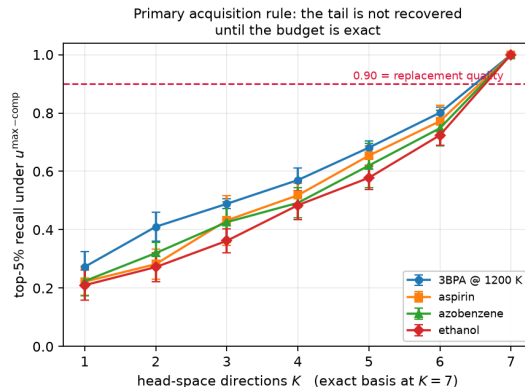
Figure 1: The negative result, under the primary max-component rule: top-5% recall against budget K on all four systems. Recall climbs steadily but never reaches the 0.90 replacement line short of the exact basis at K=7 . Error bars are the standard deviation over ten frozen seeds. Appendix B plots the corresponding screening Pareto.
