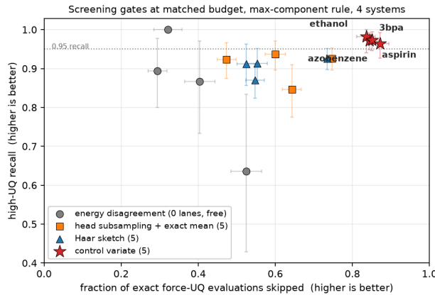
Figure 2: All four gates at matched lane budget on all four systems, under the max-component rule. Up-and-right is better on both axes, so the control variate’s dominance is read directly. Bars are 95% paired bootstrap intervals.
