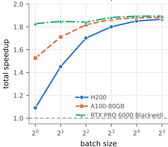
a water, 192 atoms, periodic
