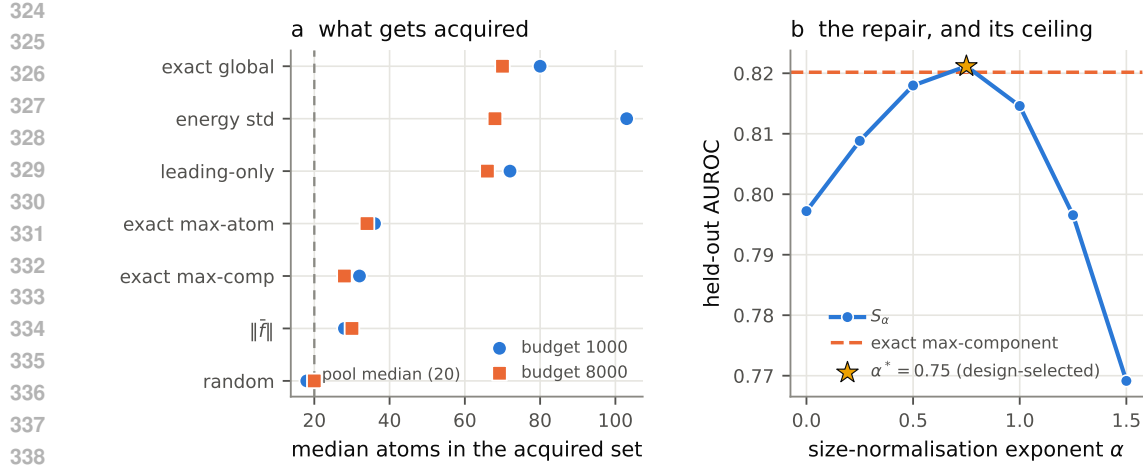
Figure 4: The global statistic is extensive, and normalisation restores parity rather than superiority. (a) Median atom count of the acquired set on the MPtraj pool. The global statistic and the two quantities that inherit its extensivity acquire far larger structures than the pool median; the intensive statistics and the free signal do not. (b) Held-out AUROC of S_\alpha = (\sum_d v_d)/(3N)^\alpha against the exponent \alpha , with the design-selected \alpha^* starred. The curve peaks near max-component’s level, not above it.
