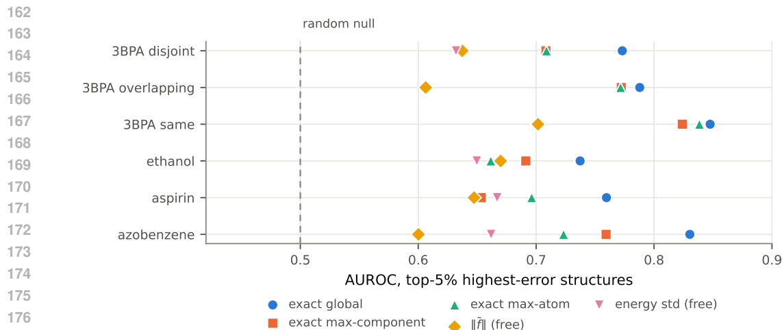
Figure 1: Exact committee disagreement ranks reference-force error, and the global statistic ranks it best at fixed system size. AUROC for detecting the top-5% highest-error structures, by signal, on the six molecular systems. The dashed line is the random null; every signal carries a distinct marker so the comparison survives grayscale printing. The two free signals cost no backward pass, and the margin over the better of them is 0.067–0.182 AUROC.
