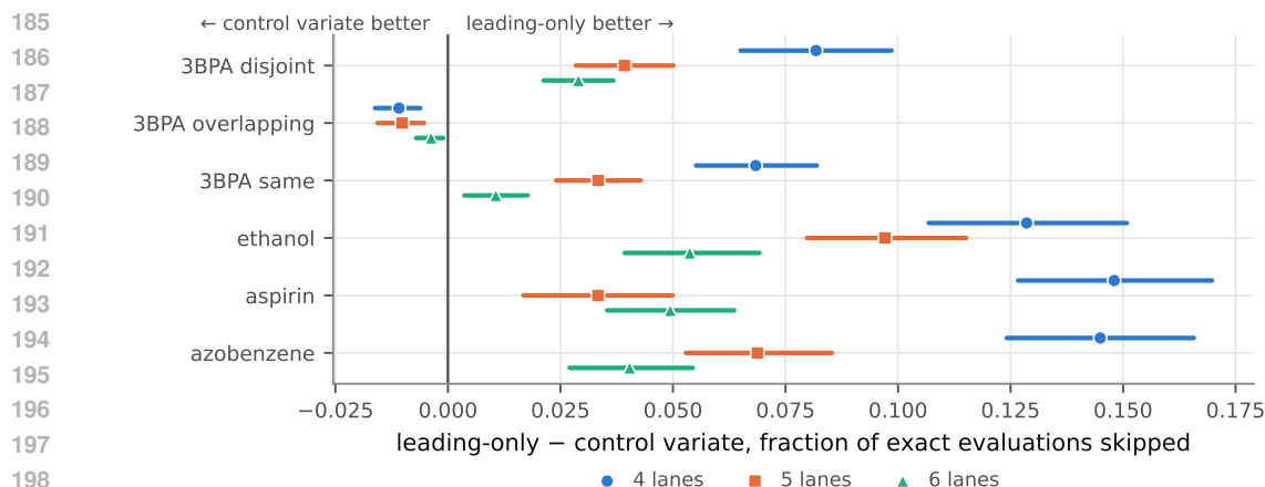
Figure 2: Randomisation does not earn its lanes. Difference in the fraction of exact evaluations skipped between the deterministic leading-only estimator and the randomised control variate, at three matched lane budgets, with 95% paired block-bootstrap intervals. Positive is leading-only better. It wins significantly on 5 of 6 systems at every budget; the single exception is 3BPA overlapping, in a regime where both estimators already skip more than 93%.
