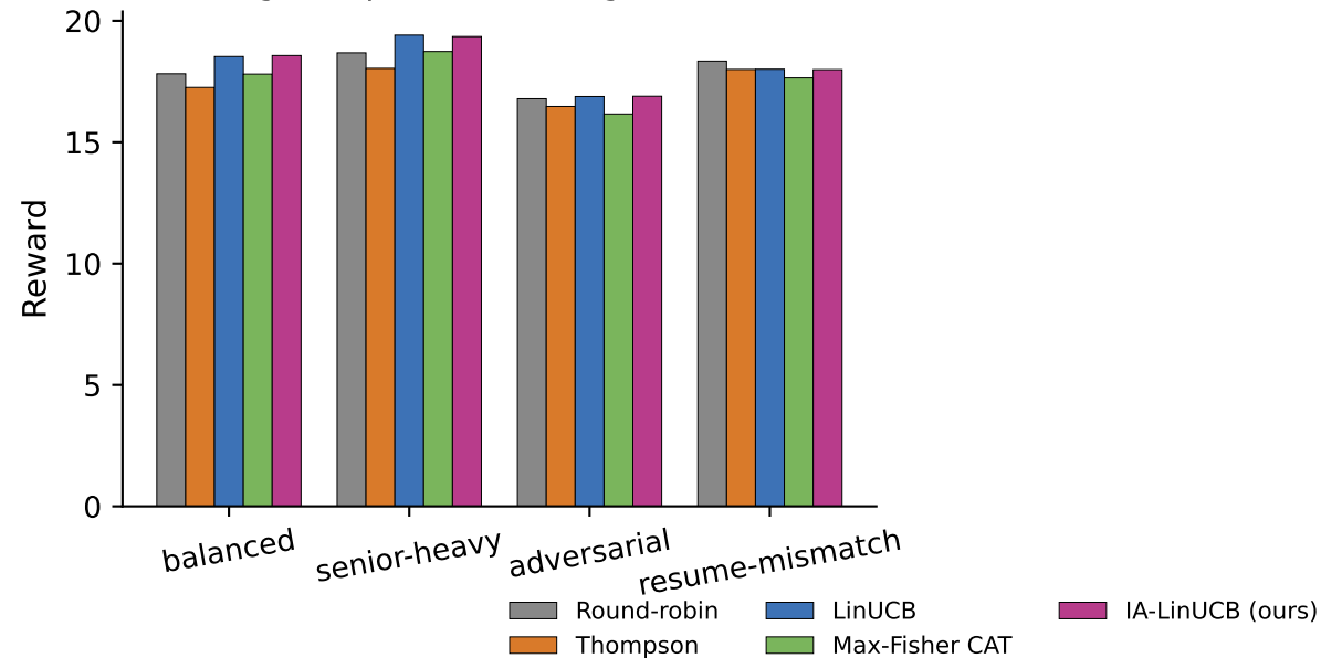
Average shaped reward (higher is better)
