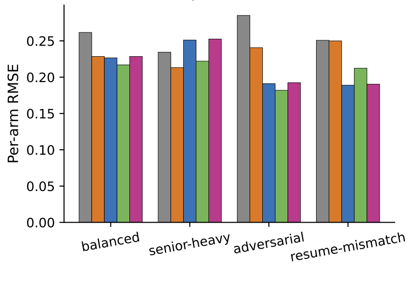
Per-arm ability RMSE (lower is better)
