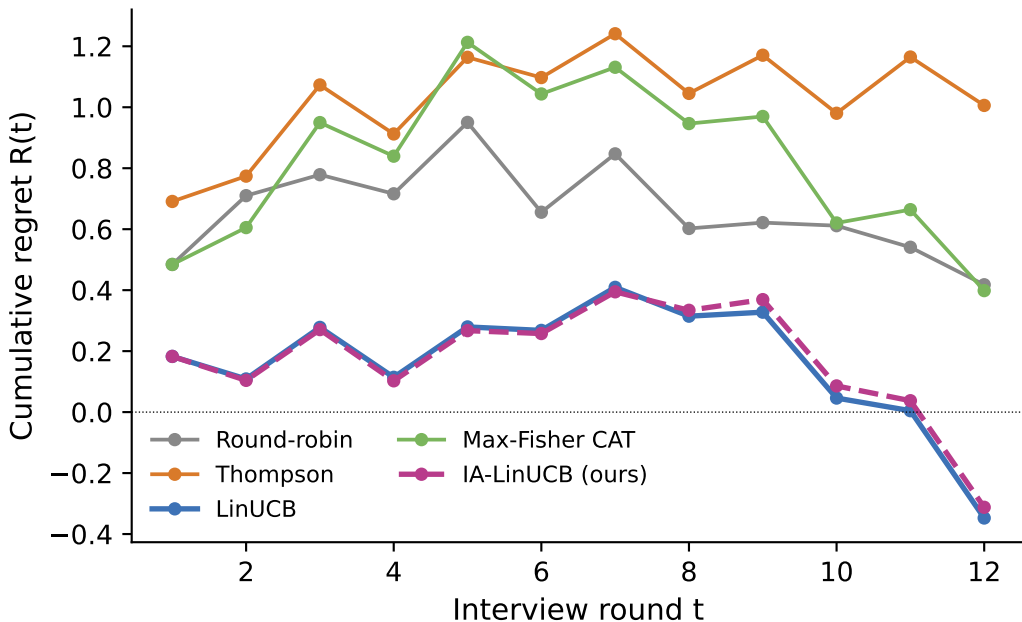
Selection-policy regret on synthetic candidates
