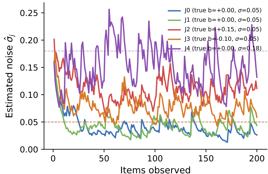
Per-judge noise estimate vs. items
