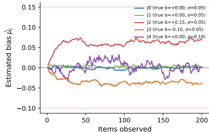
Per-judge bias estimate vs. items
