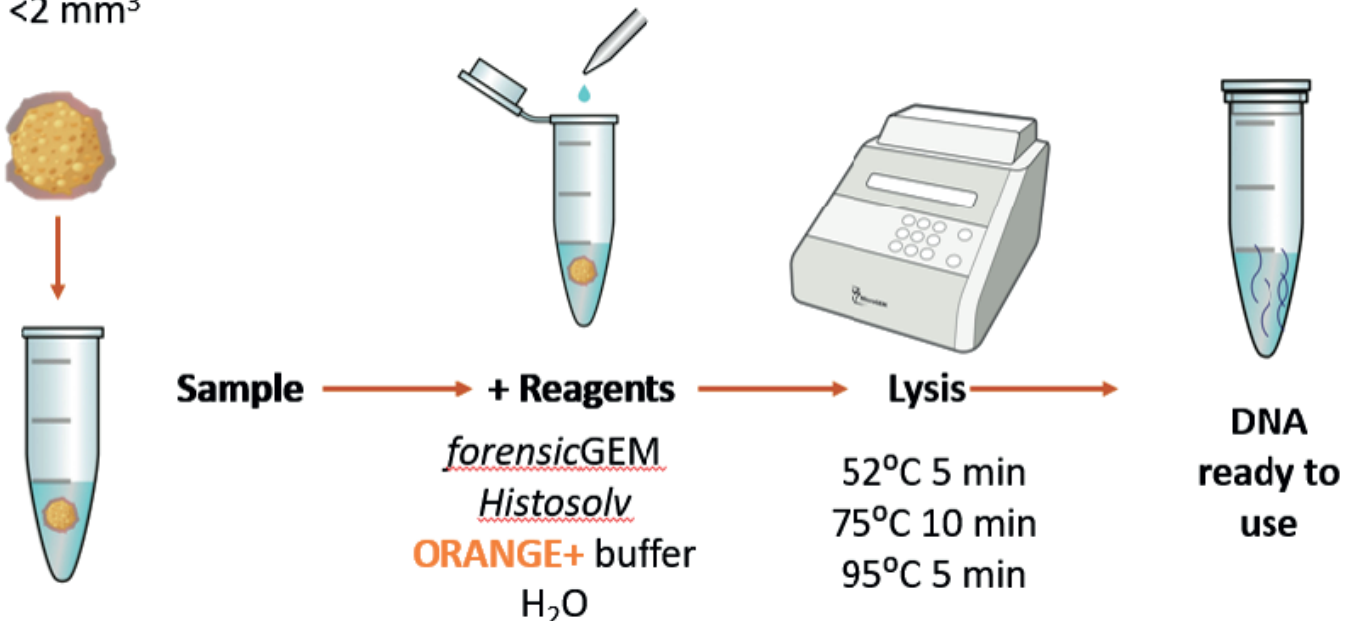
Figure 8. Workflow for DNA extraction from tissue samples.
