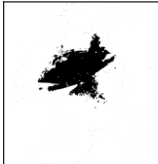
Attention U-Net
