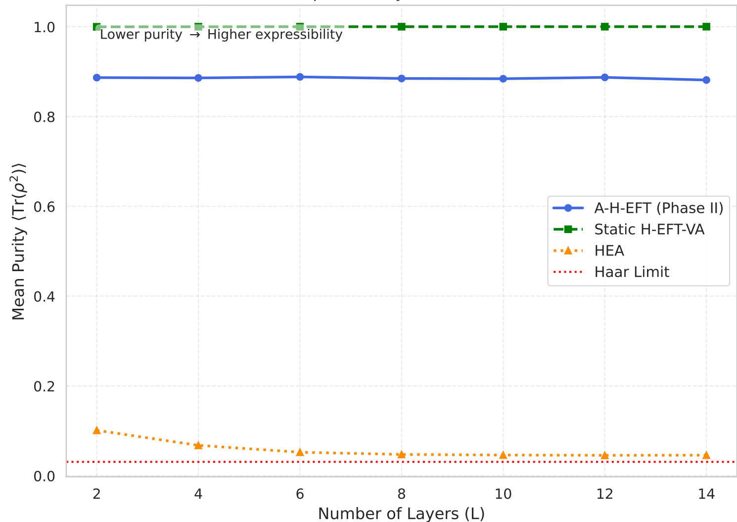
AT10: Expressibility Benchmark (N=6)
