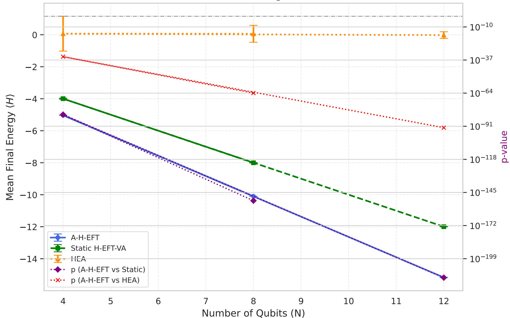
AT15: Statistical Significance
