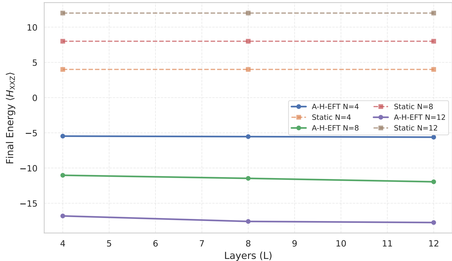
AT16: Heisenberg Convergence
