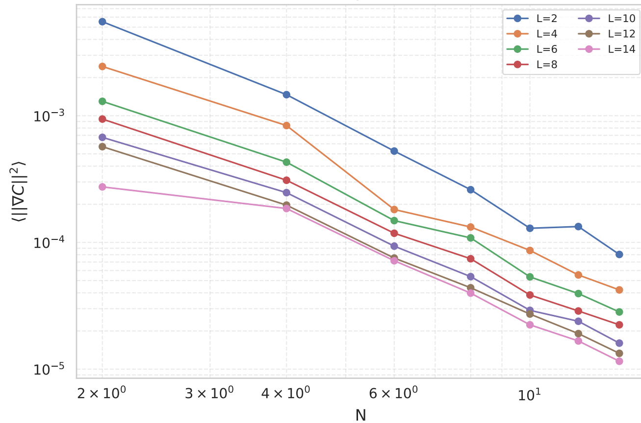
AT16 Heisenberg: Phase I (Static)
