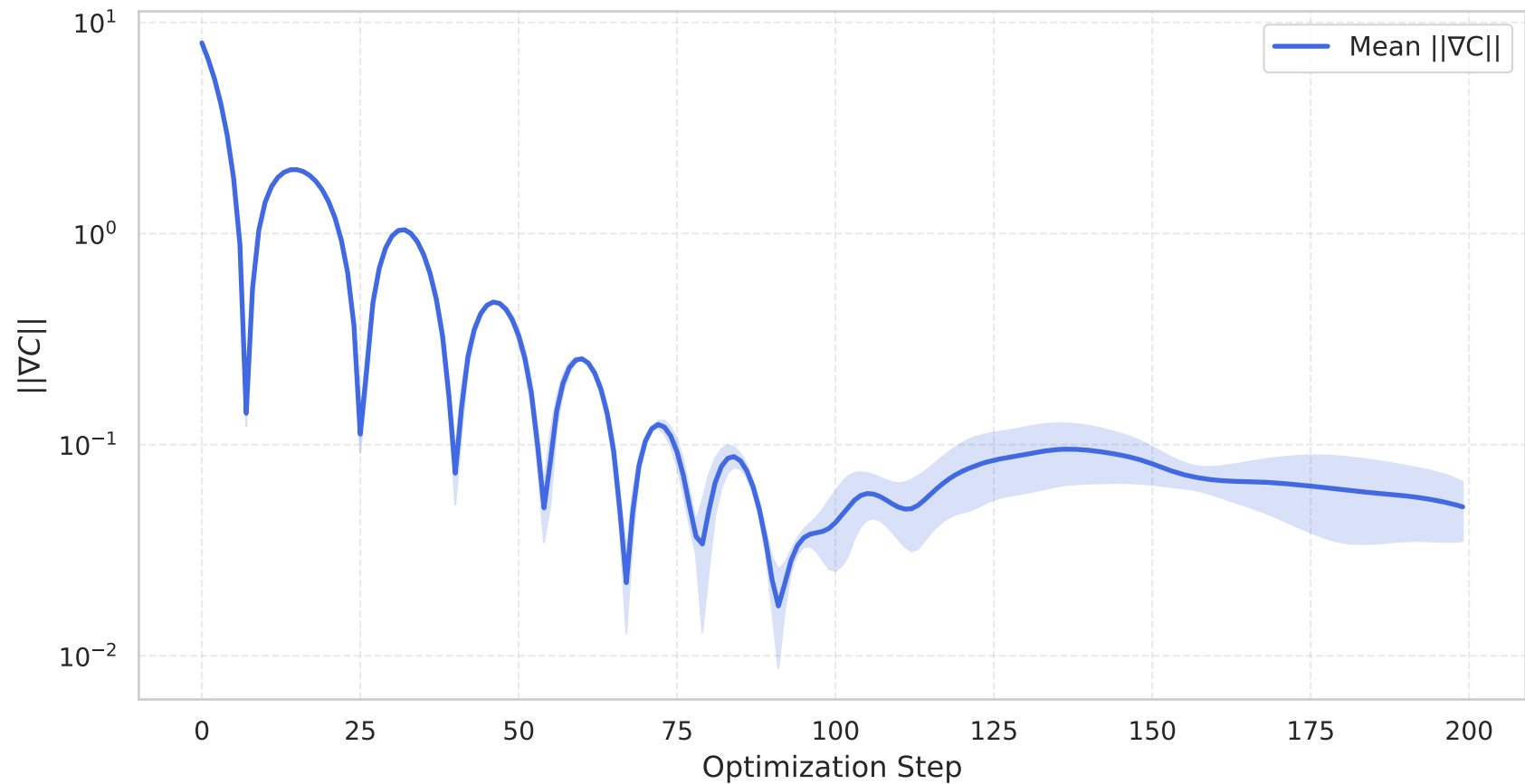
AT3: Gradient Norm Across Phase I \rightarrow Phase II
