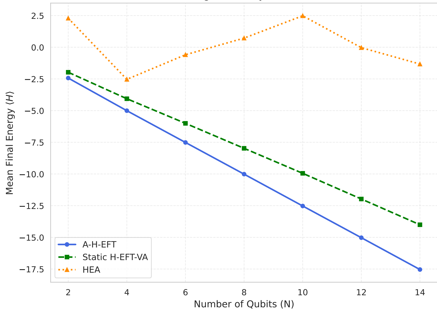
AT5: Convergence vs System Size (L=2)
