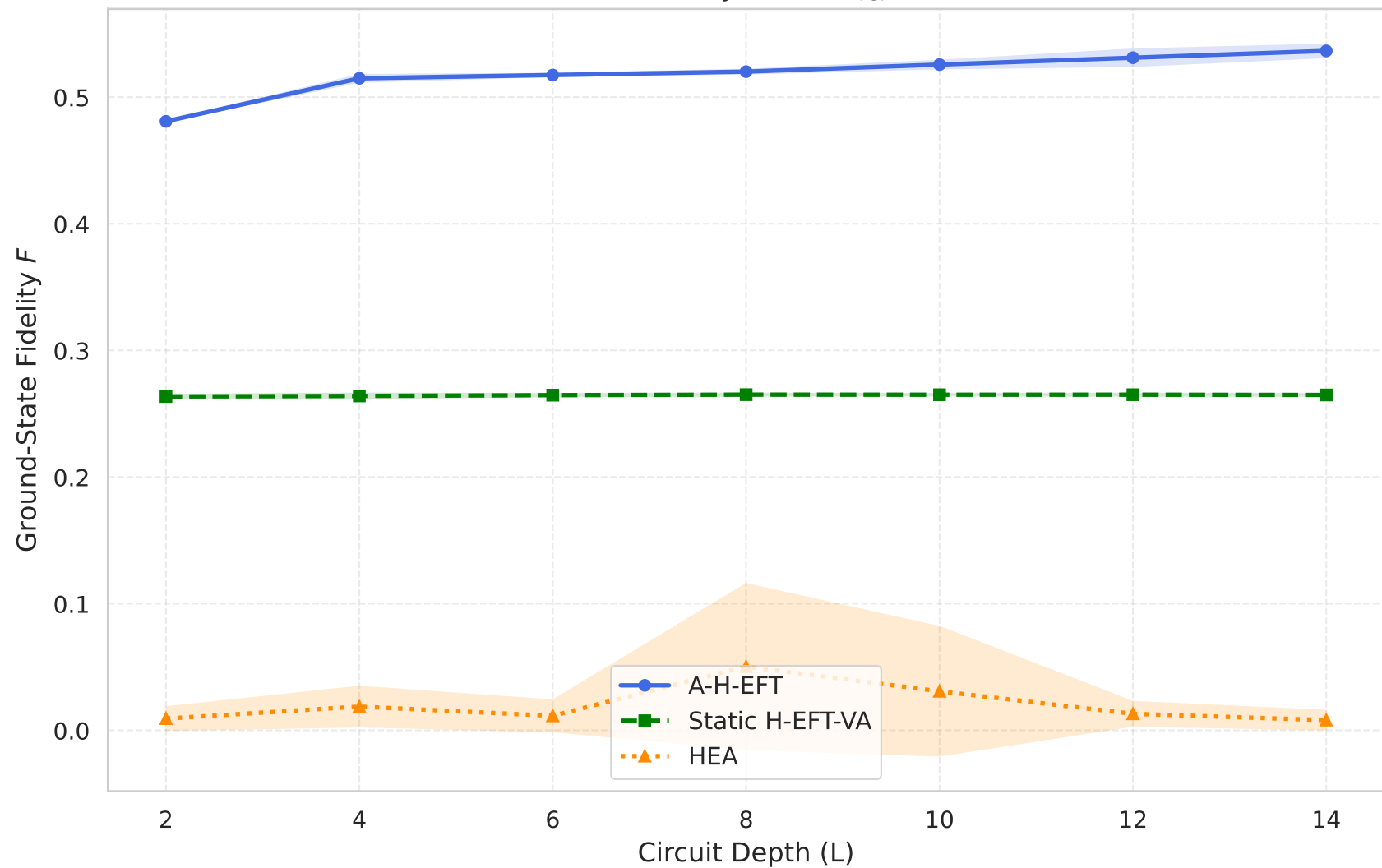
AT6: VQE Fidelity ( N=6 , \Delta_{\text{ref}}=0.736 )
