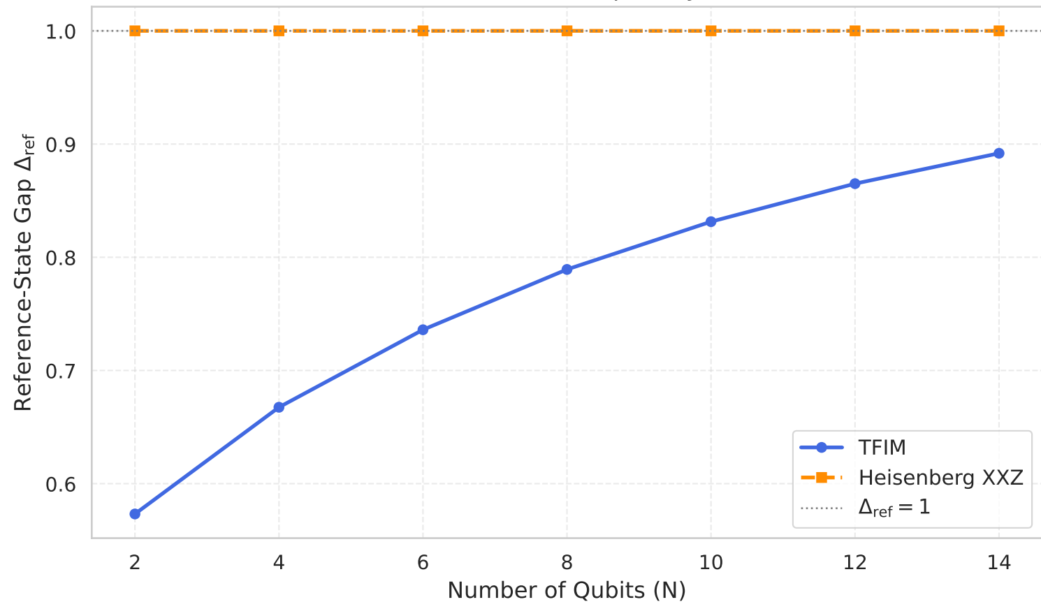
AT7: Reference-State Gap vs System Size
