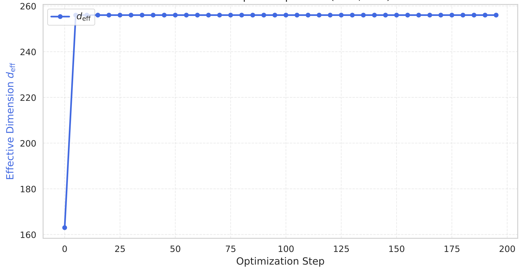
AT8: Hilbert Space Expansion (N=8, L=8)
