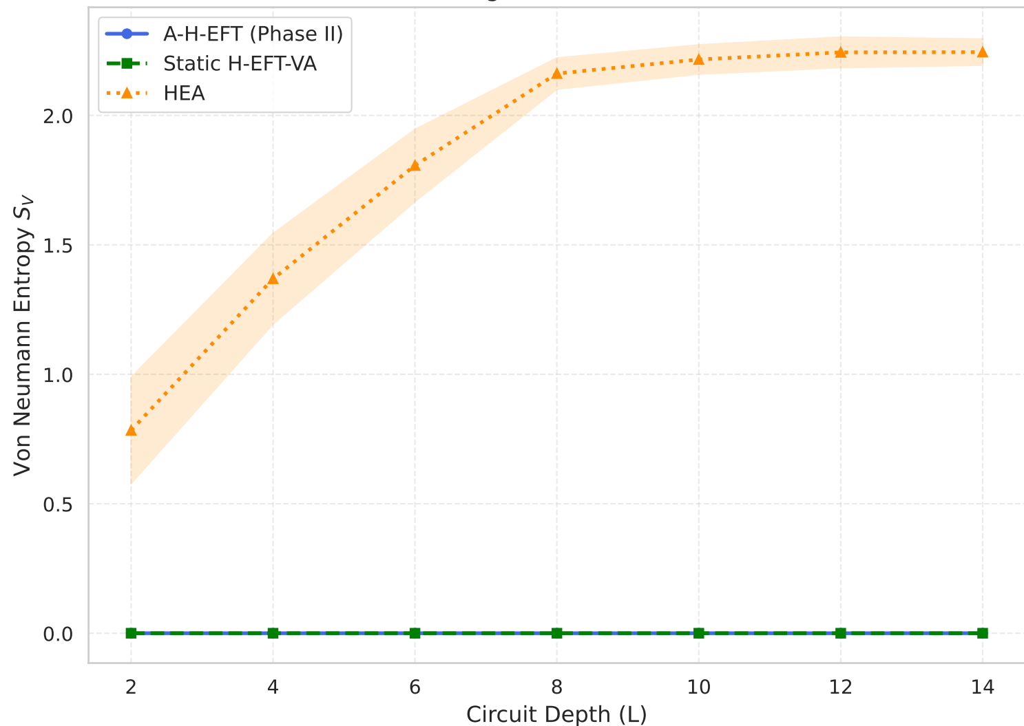
AT9: Entanglement Growth (N=8)
